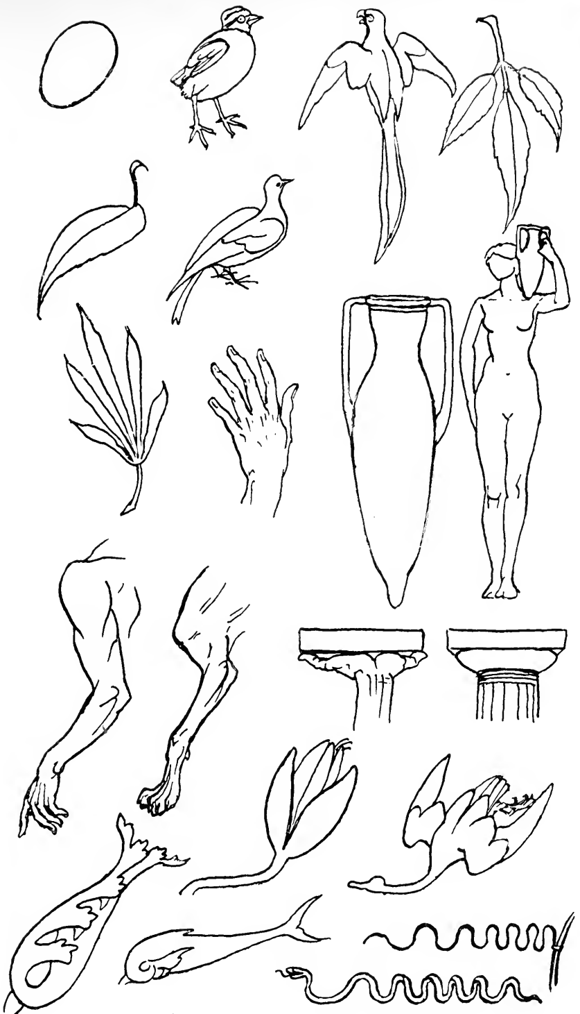
SOME ANALOGIES IN FORM.
